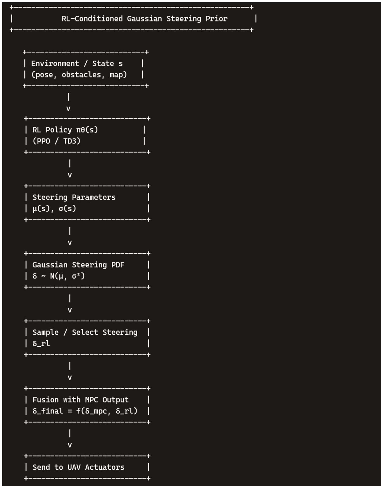
Fig.5. RL-conditioned Gaussian steering prior combining PPO/TD3 outputs with MPC steering.
